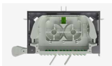
Splitter Option - Splicing Area
